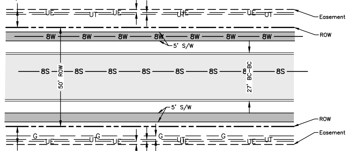
Typical Utility Layout Legend
